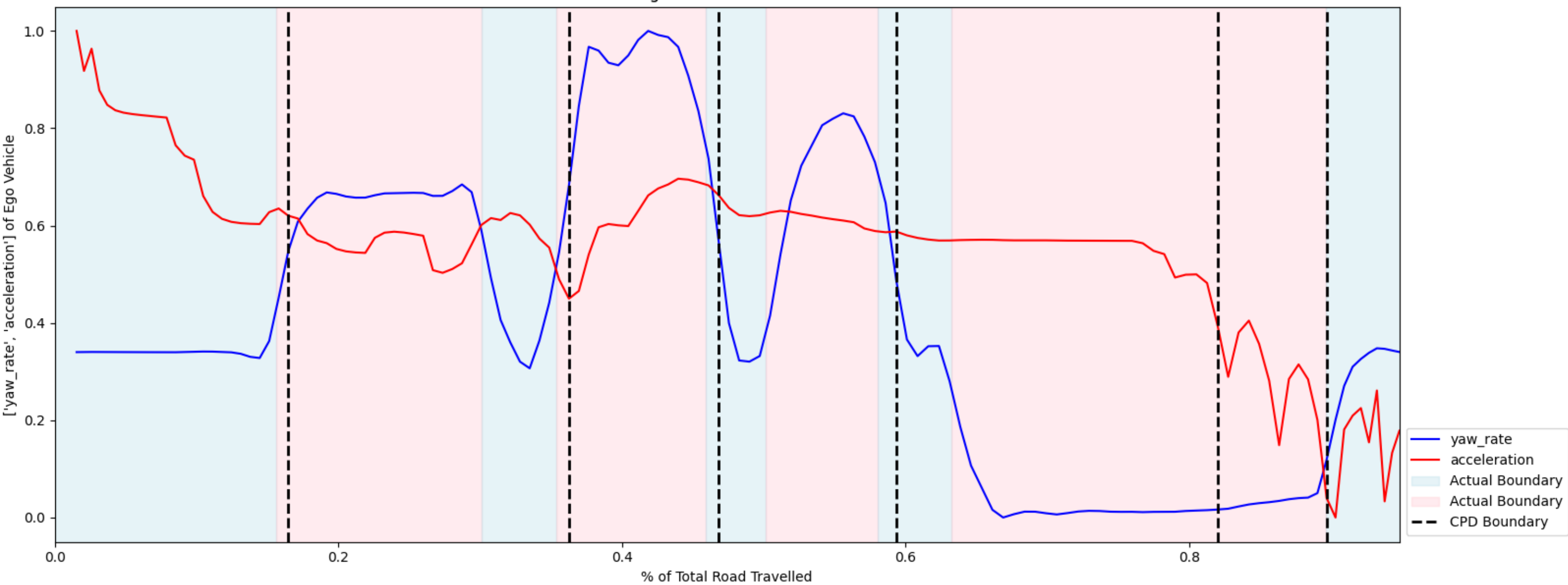
CPD Algorithm Results - Window
